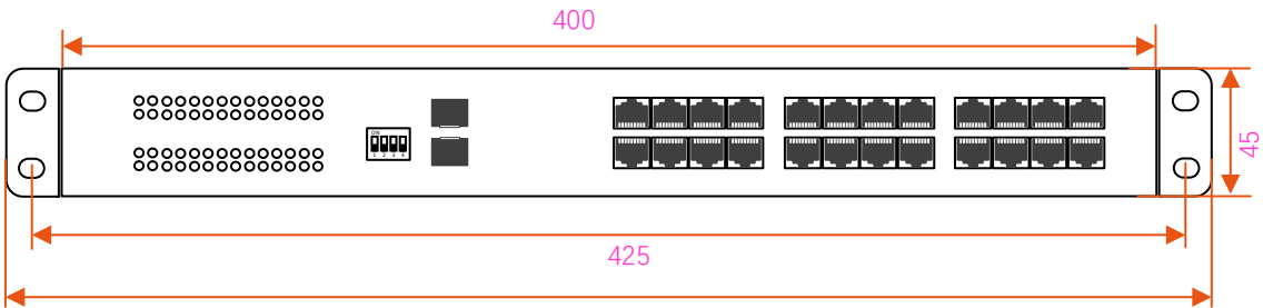
Front View
